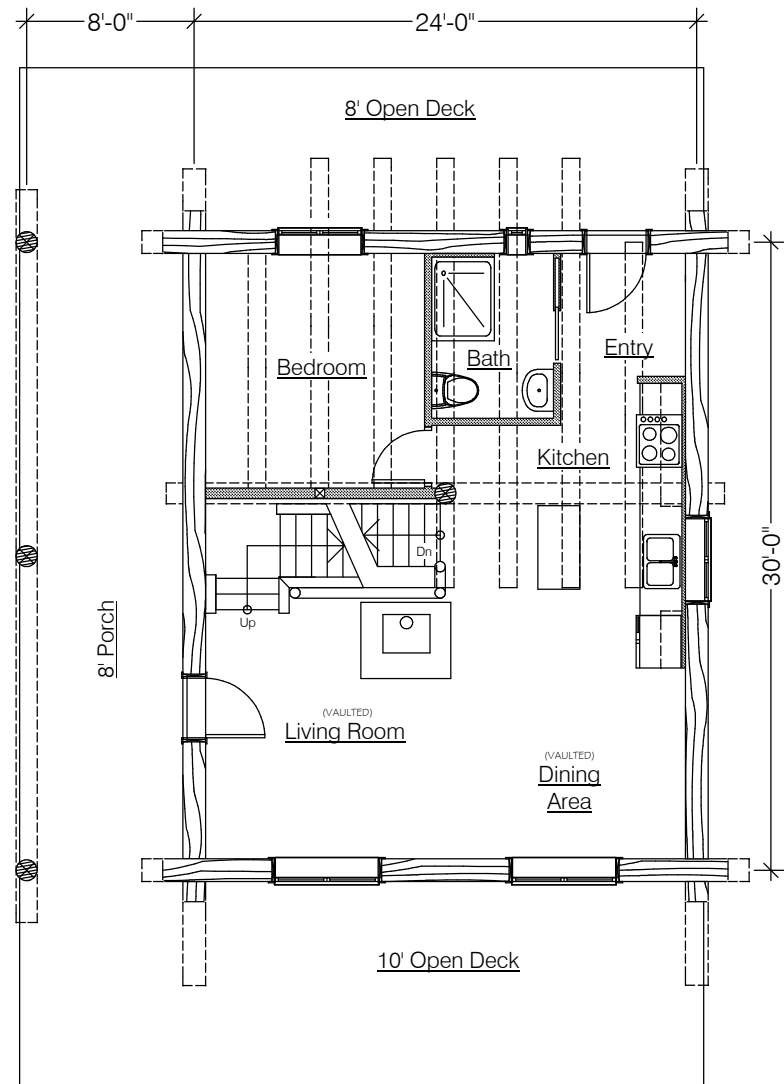
Main Floor Plan House - 756 Sq. Ft.
