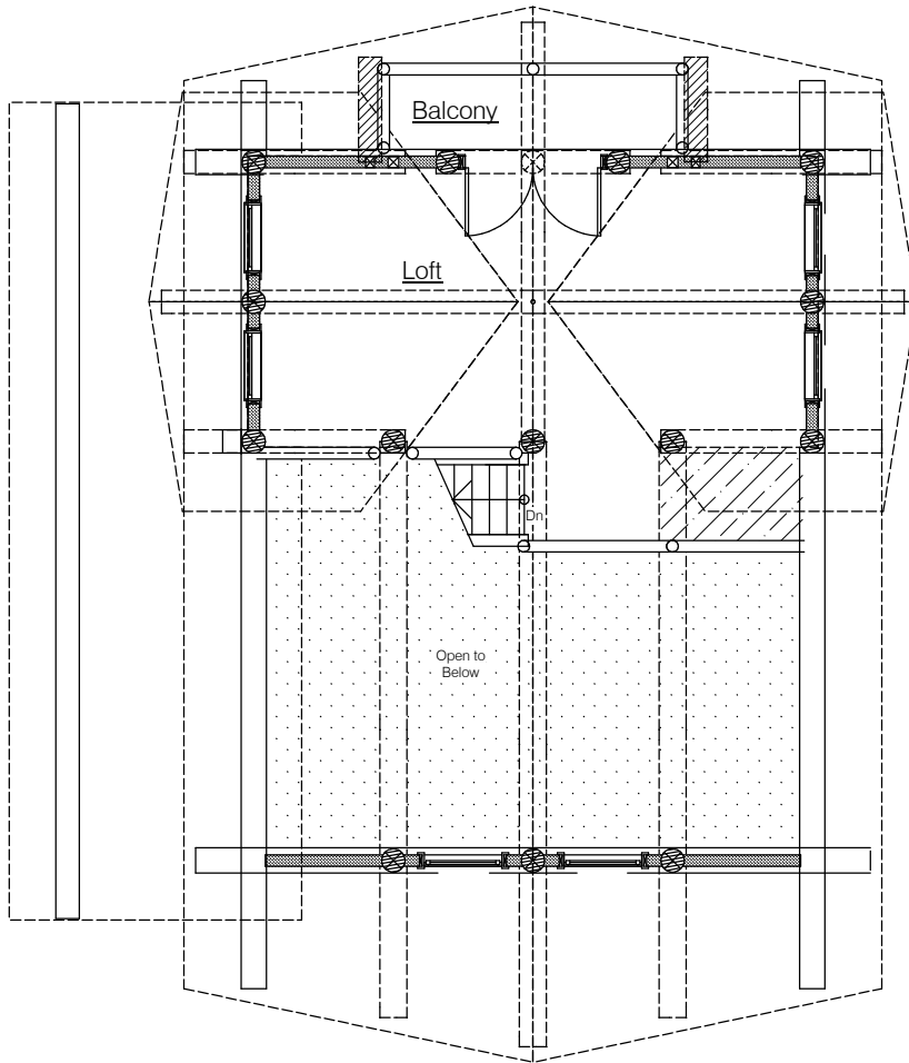
Loft Floor Plan 330 Sq. Ft. (over 6' headroom)
