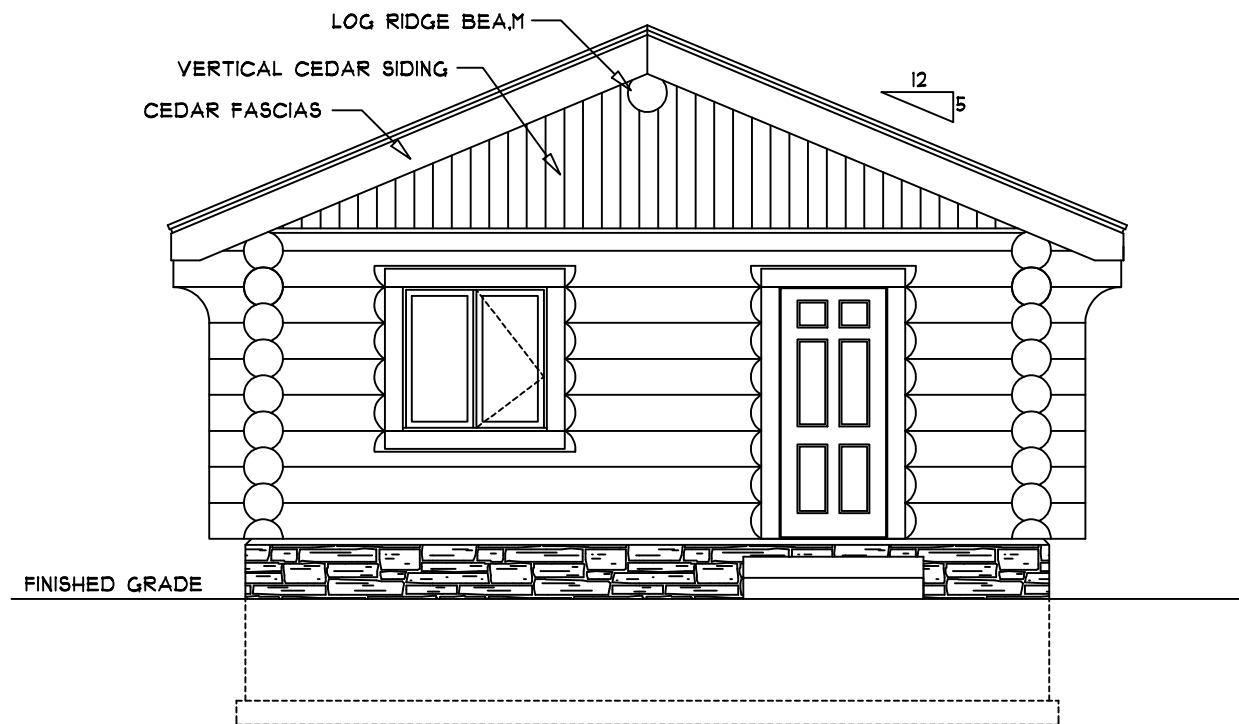
Front Elevation
