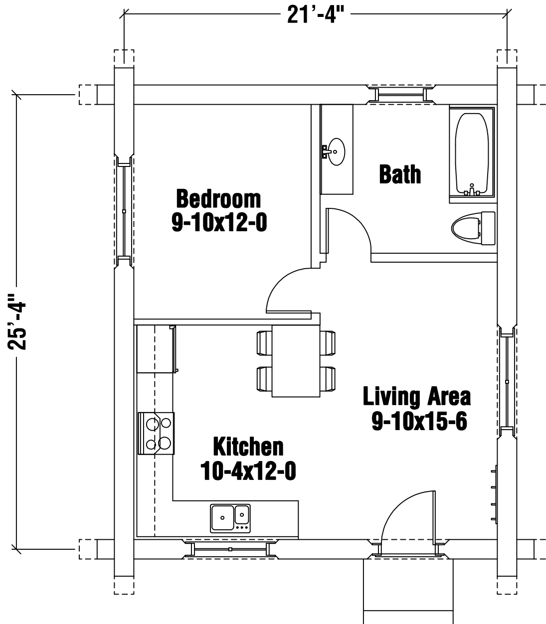
Main Floor Plan 572 SQ.FT.
