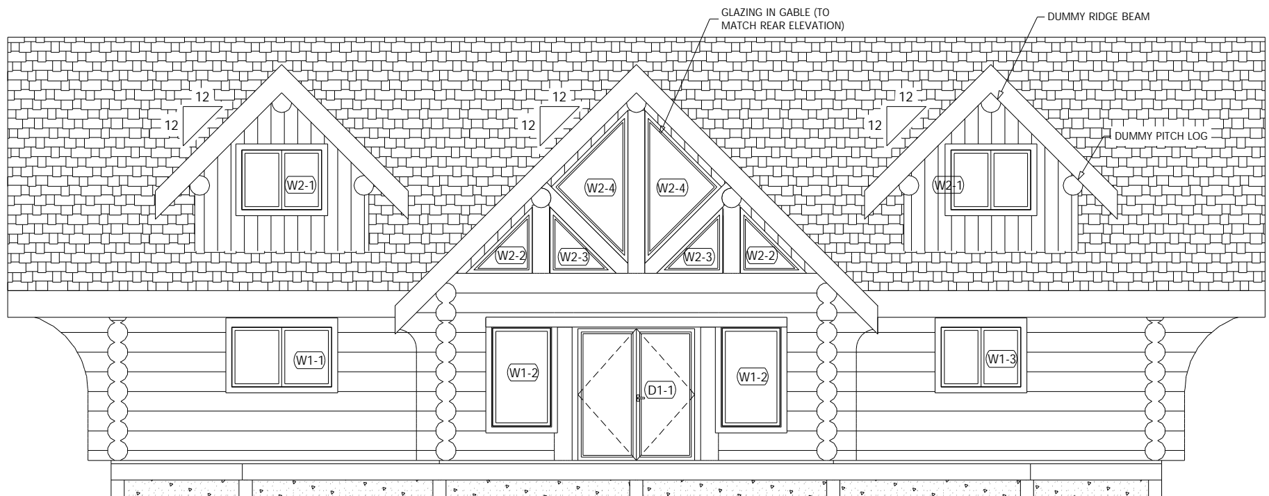
Front Elevation
