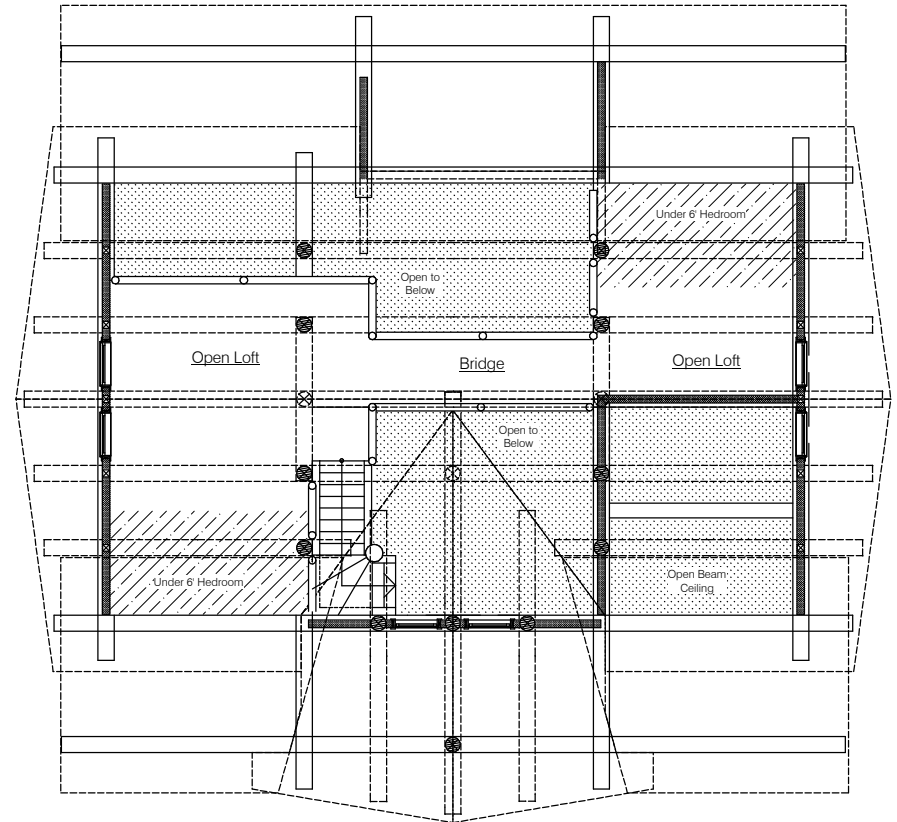
Loft Floor Plan 437 Sq. Ft. (over 6' headroom)
