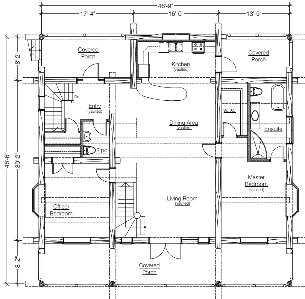
Main Floor Plan House - 1598 Sq. Ft.
