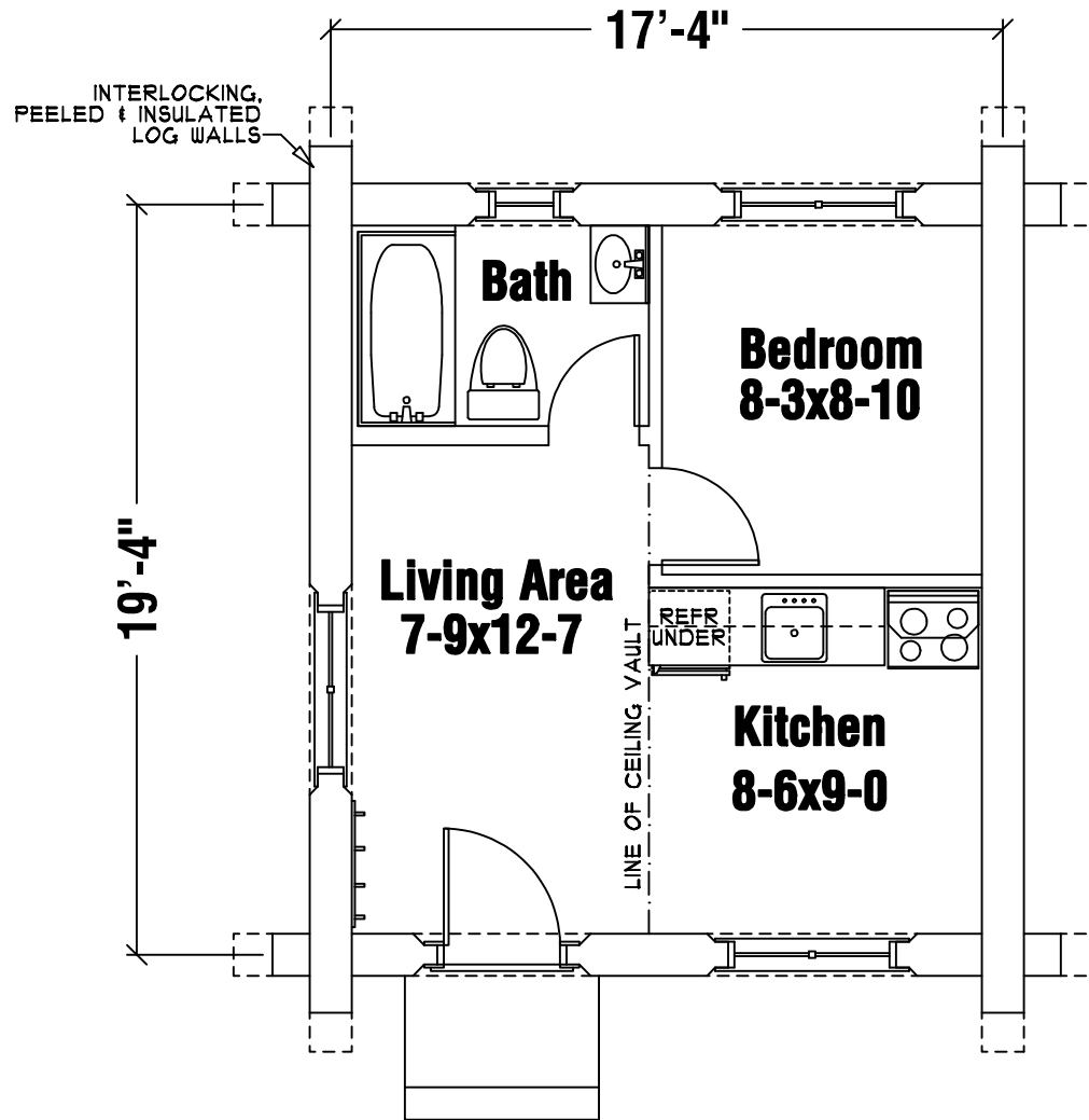
Main Floor Plan 360 SQ.FT.
