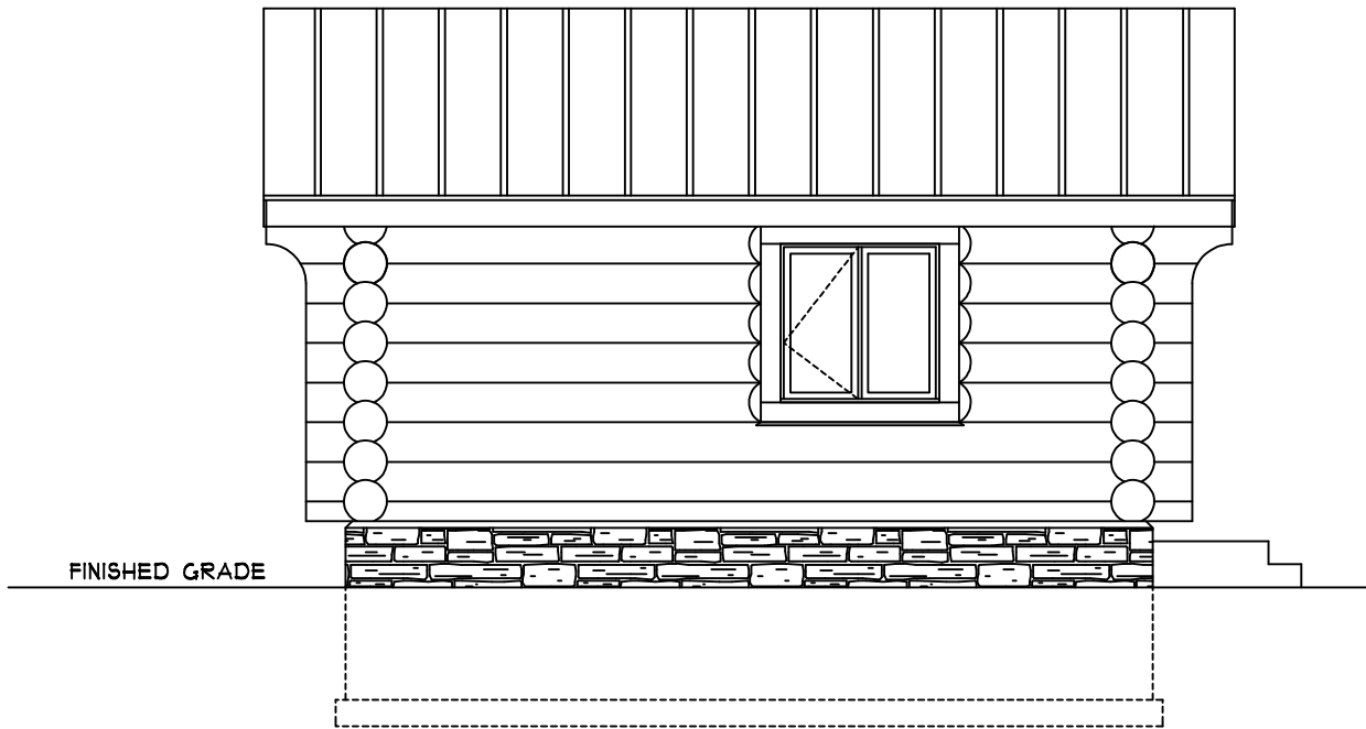
Left Elevation
