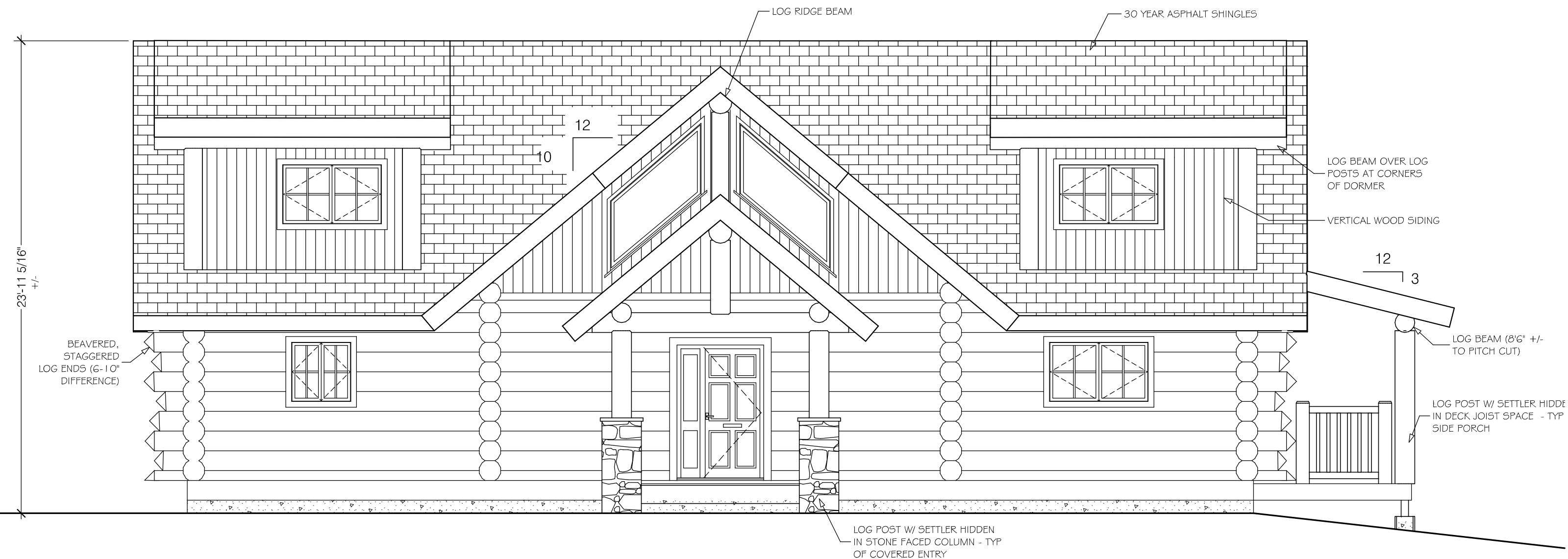
Front Elevation
